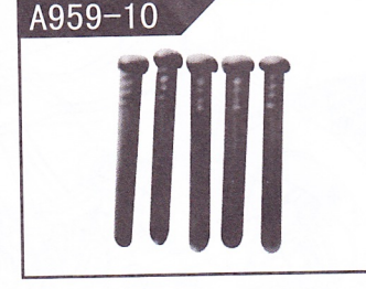
Round head screw level M2X17.5
